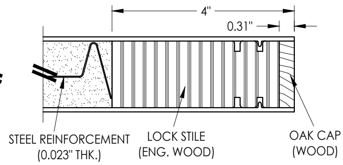
2 HORIZONTAL CROSS SECTION
