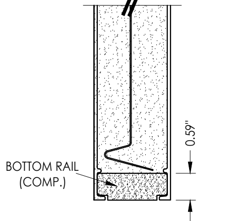
2 3 VERTICAL CROSS SECTION
